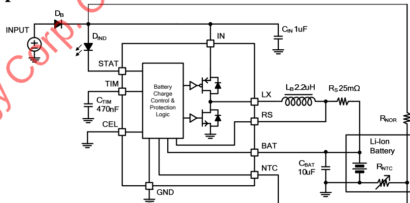
Figure 1. SY6912A Schematic Diagram
