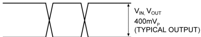
Figure 4. Single-Ended Swing
