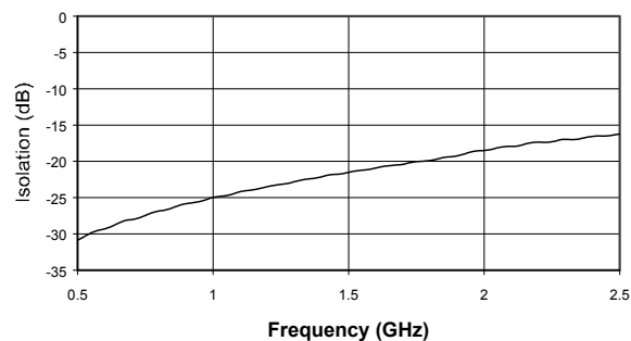
Isolation vs. Frequency, 25 °C, 100 pF
