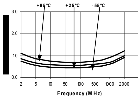
Insertion Loss
