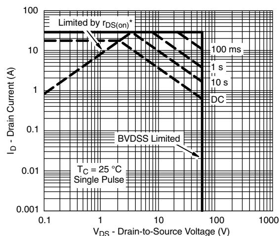
* V_{GS} > minimum V_{GS} at which r_{DS(on)} is specified
