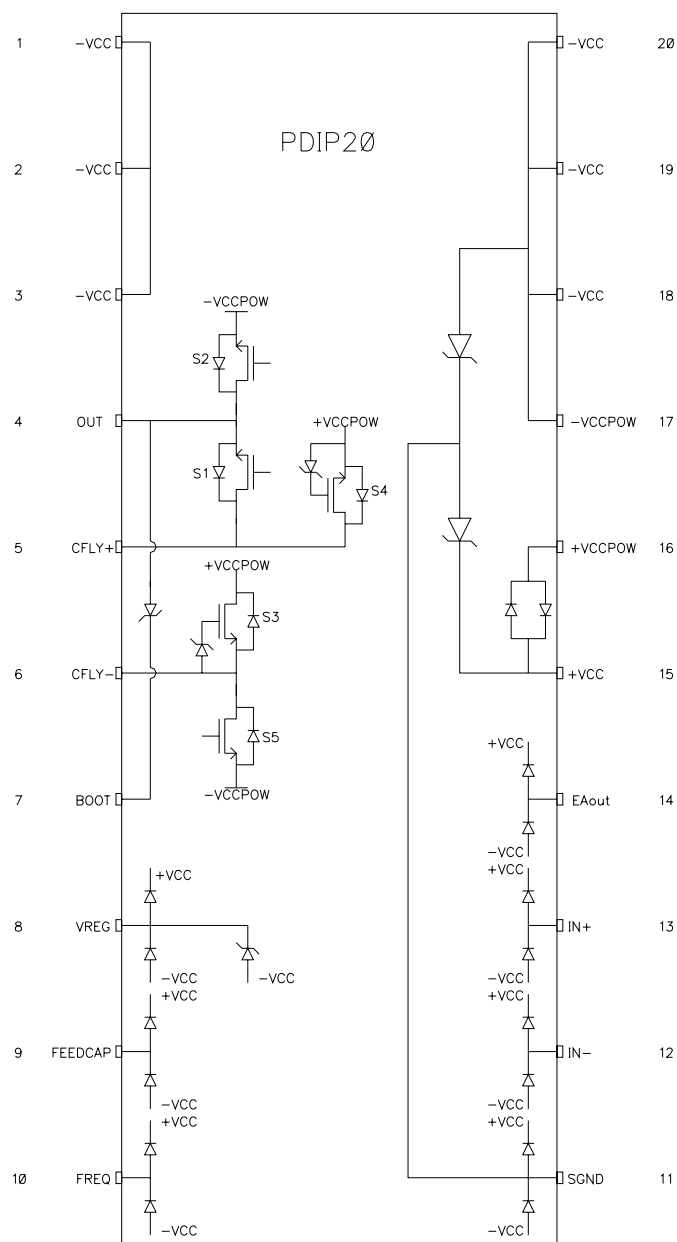
Figure 8: ESD Protection Structure
