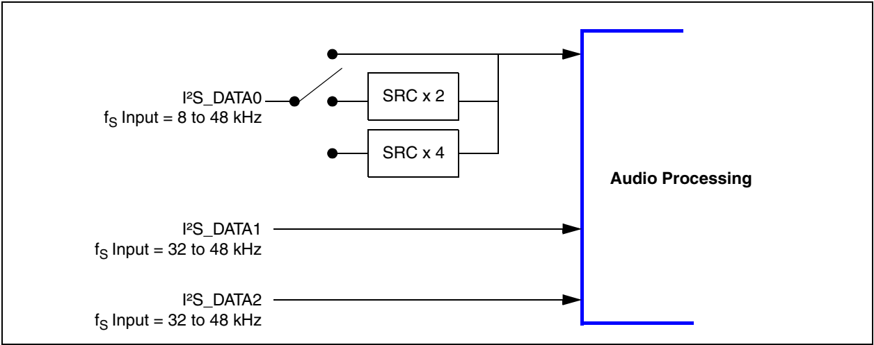
Figure 25: I²S Block Diagram
