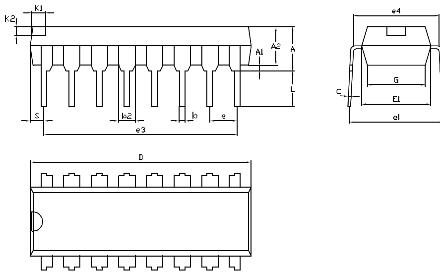
Figure 10: 16-Pin Plastic Dual In-Line Package, 300-mil Width
