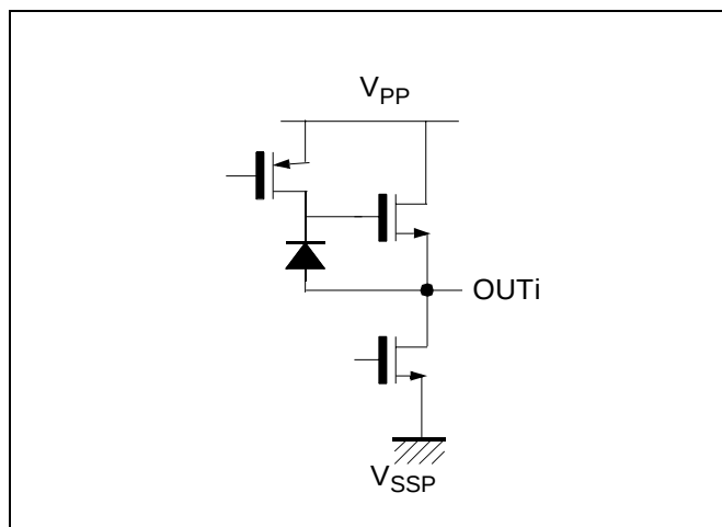
Figure 8: Power Outputs
