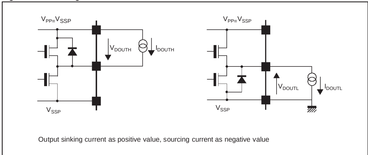
Figure 4. Test configuration
