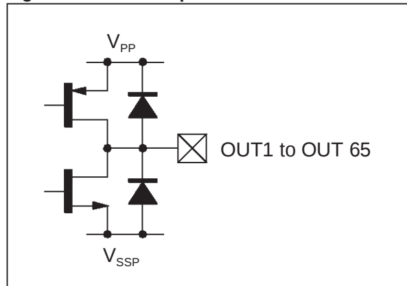
Figure 6: Power Output
