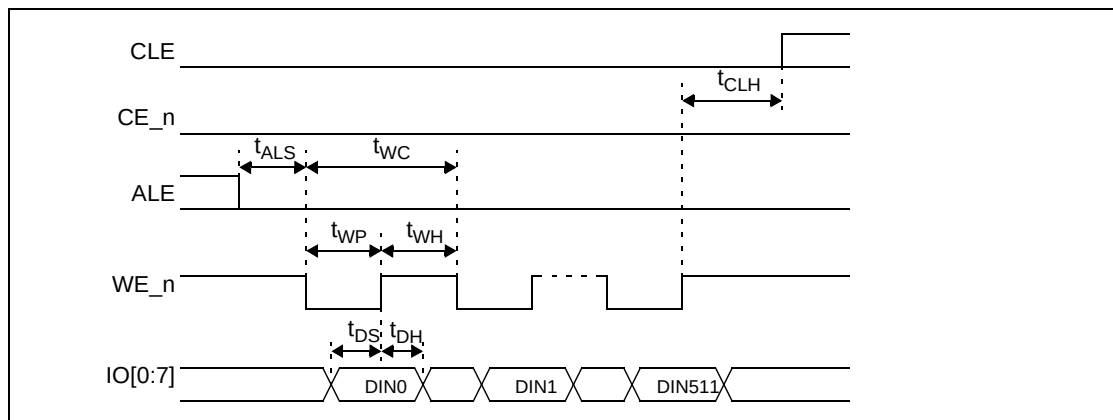
Figure 14: Input data latch cycles for NAND flash interface
