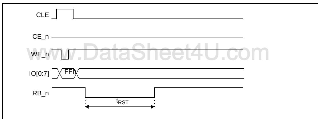
Figure 18: Reset operation for NAND flash interface
