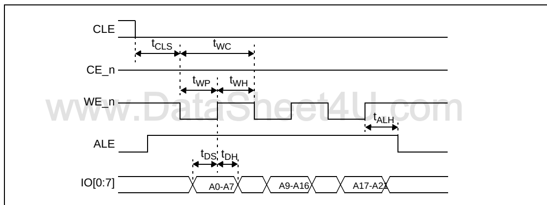
Figure 13: Address latch cycle for NAND flash interface
