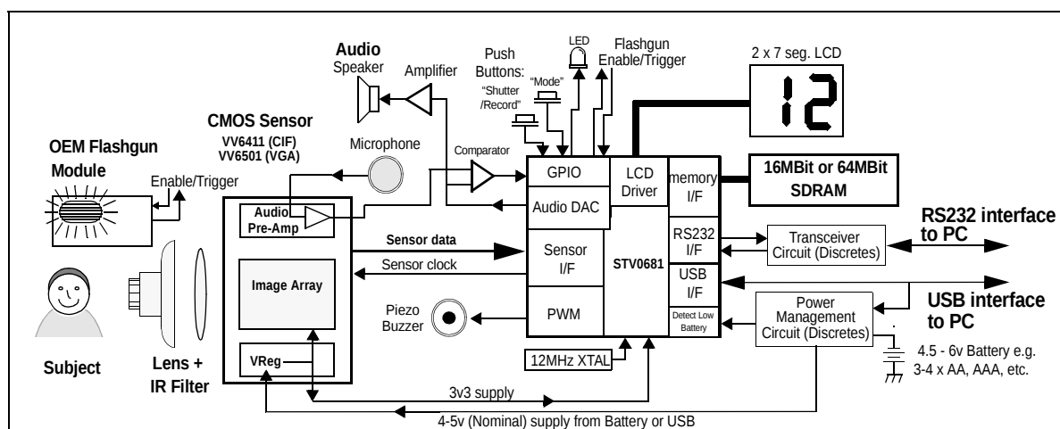
Figure 1: Typical camera system block diagram
