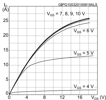
Figure 6: Output characteristics
