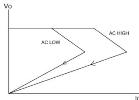
Figure 9. Current-mode control
