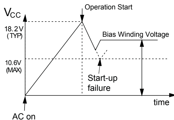
Figure 4. VCC pin voltage after start-up, capacitor C3 installed
