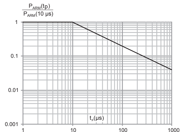
Figure 6. Normalized avalanche power derating versus pulse duration ( T_j = 125 °C)
