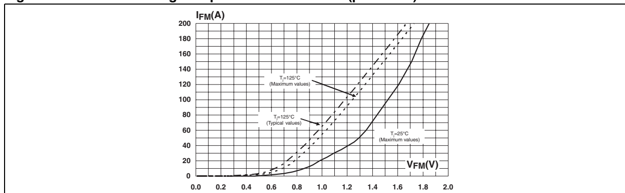
Figure 11. Forward voltage drop vs. forward current (per diode)
