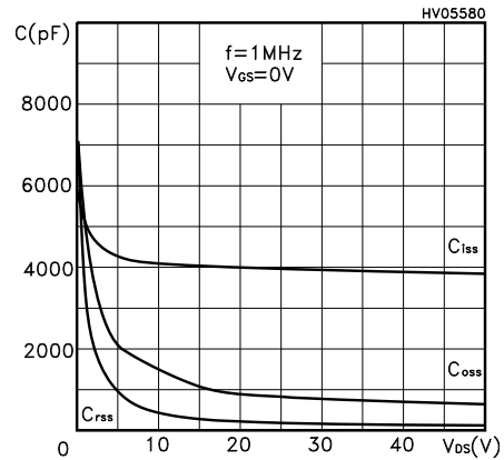
Figure 9. Capacitance variations
