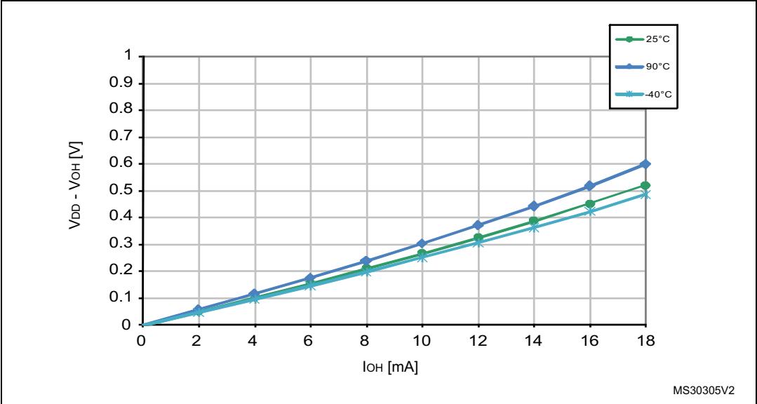
Figure 22. Typ. V_{DD} - V_{OH} at V_{DD} = 3.0\text{ V} (standard ports)
