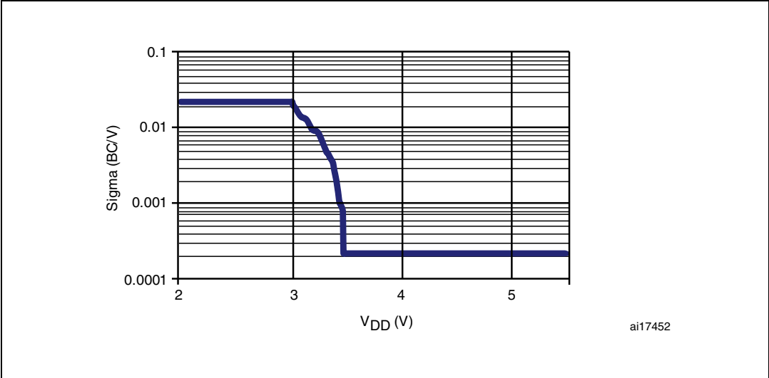
Figure 23. Sigma variation across V_{DD}
