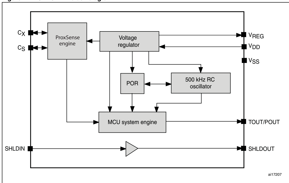
Figure 1. STM8T141 block diagram
