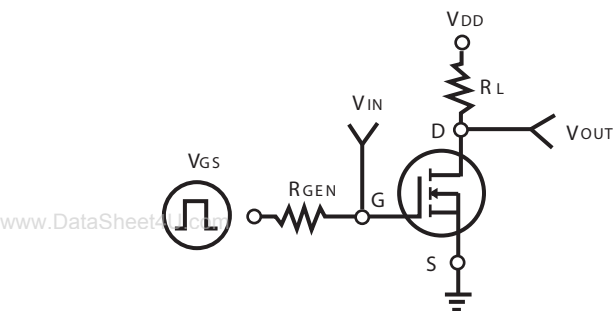
Figure 11. Switching Test Circuit
