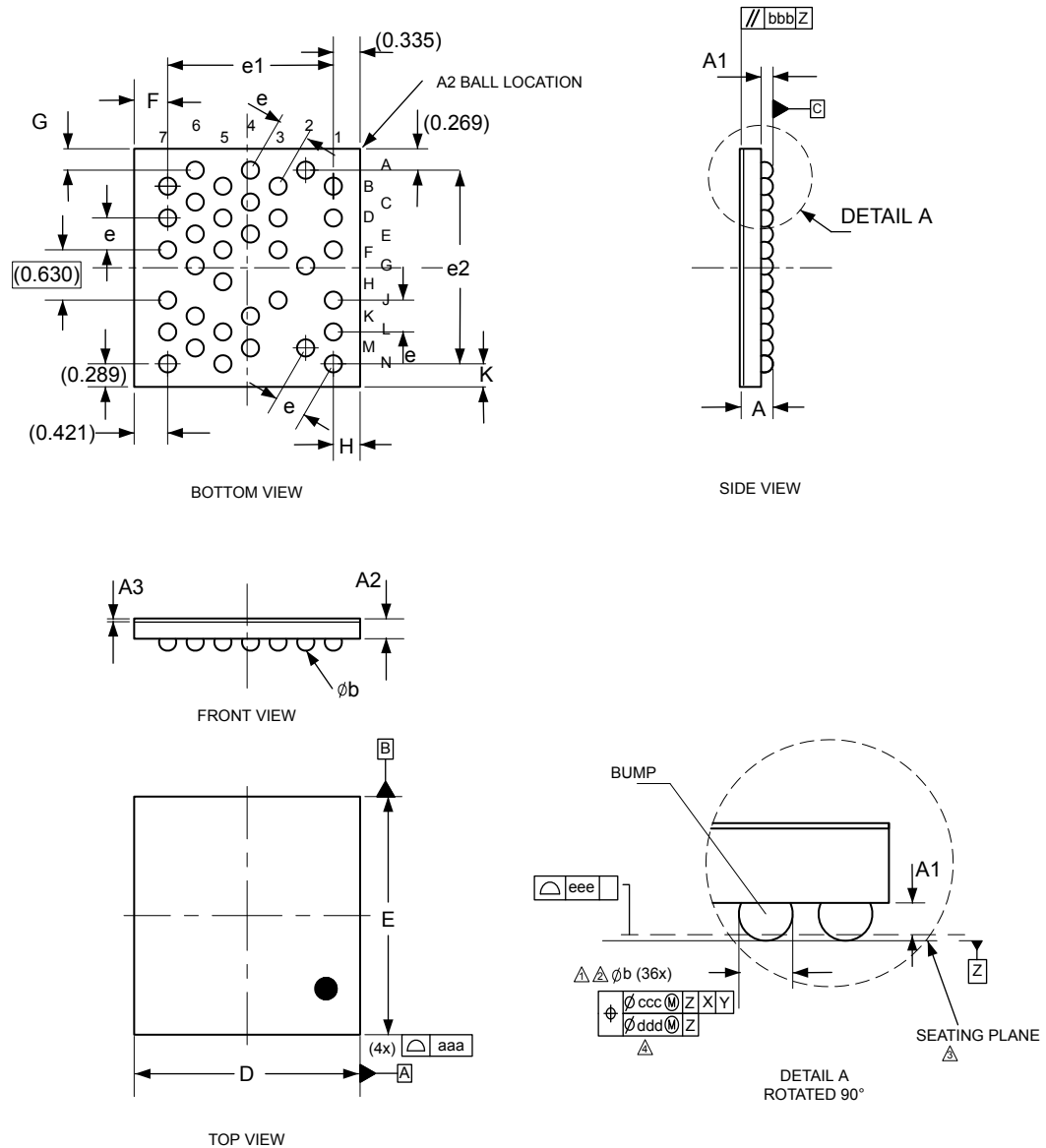
Figure 19. WLCSP36 - Outline
