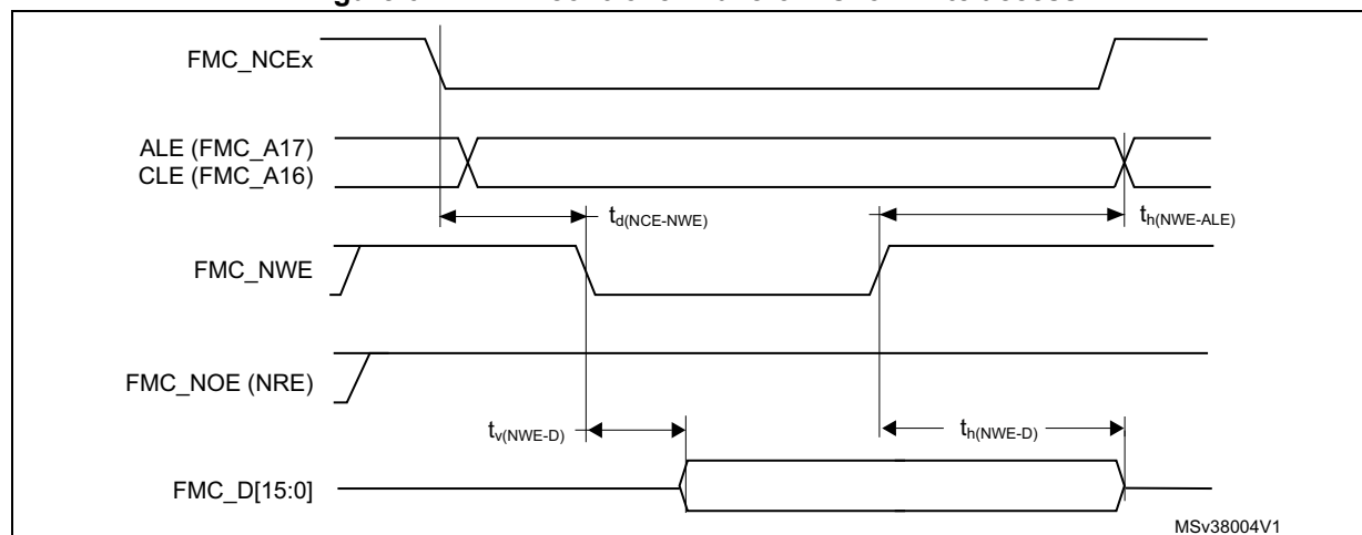
Figure 64. NAND controller waveforms for write access
