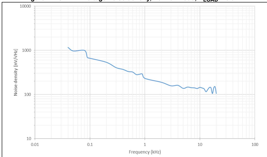
Figure 44. OPAMP voltage noise density, normal mode, R_{LOAD} = 3.9\text{ k}\Omega
