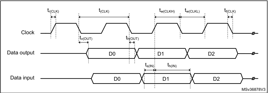
Figure 73. HSPI timing diagram - SDR mode
