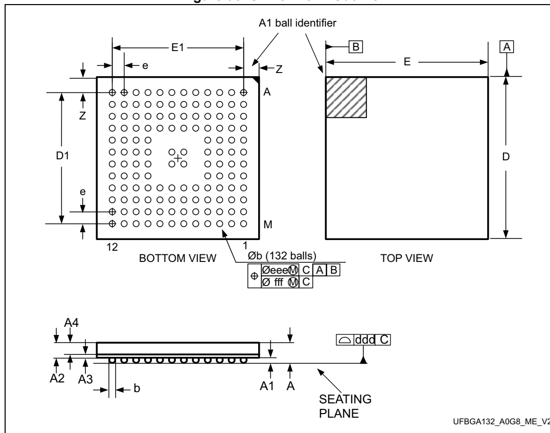
Figure 96. UFBGA132 - Outline
