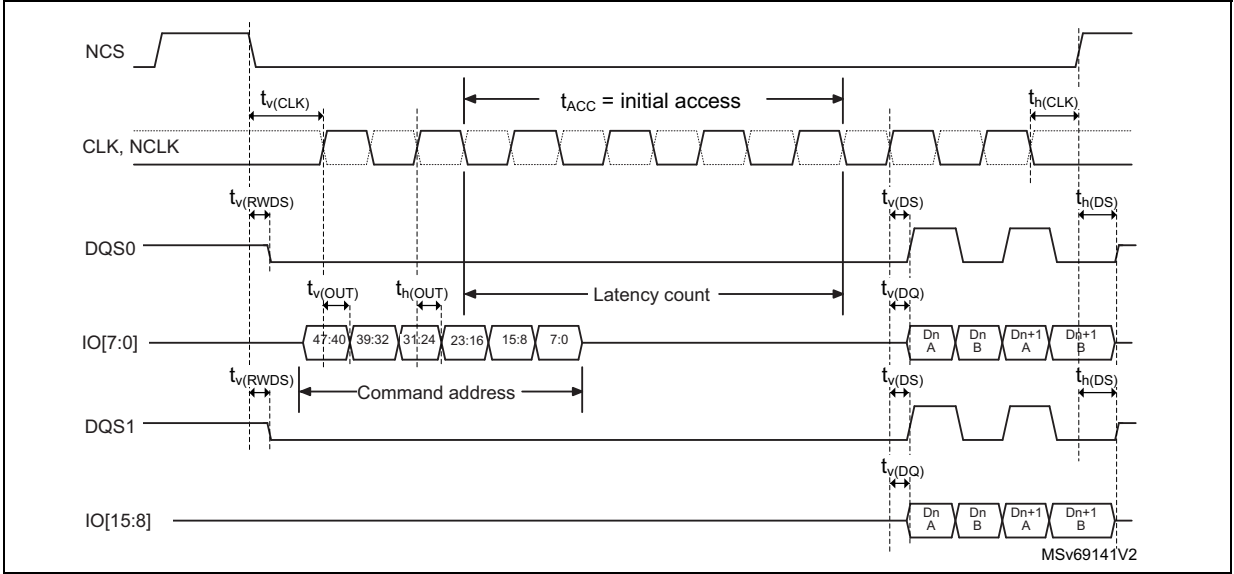
Figure 76. HSPI HyperBus read
