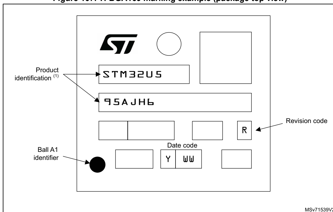
Figure 107. TFBGA169 marking example (package top view)
