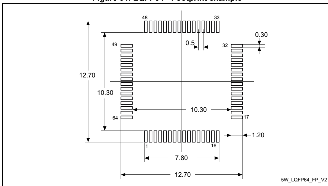
Figure 91. LQFP64 - Footprint example
