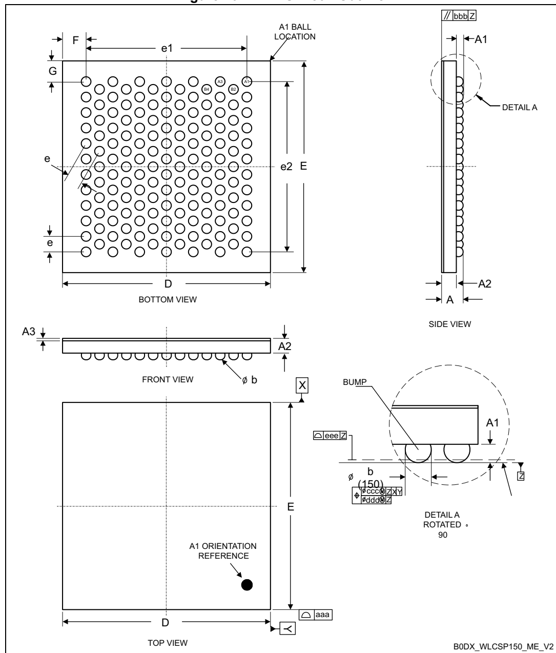
Figure 102. WLCSP150 - Outline
