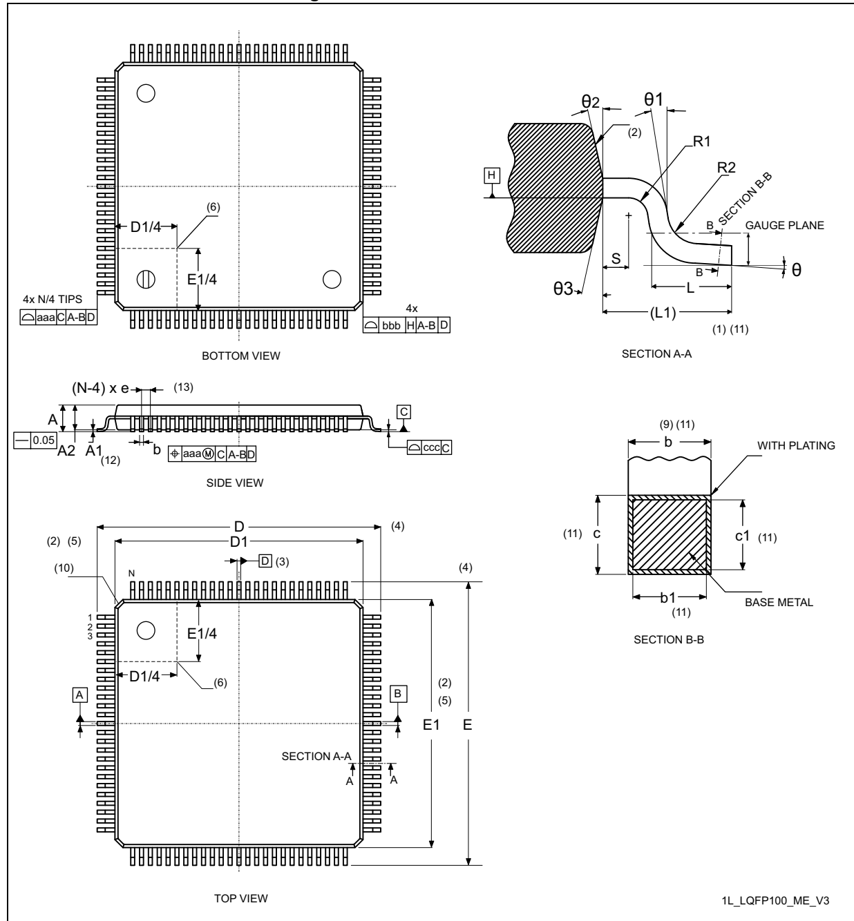
Figure 93. LQFP100 - Outline (15)
