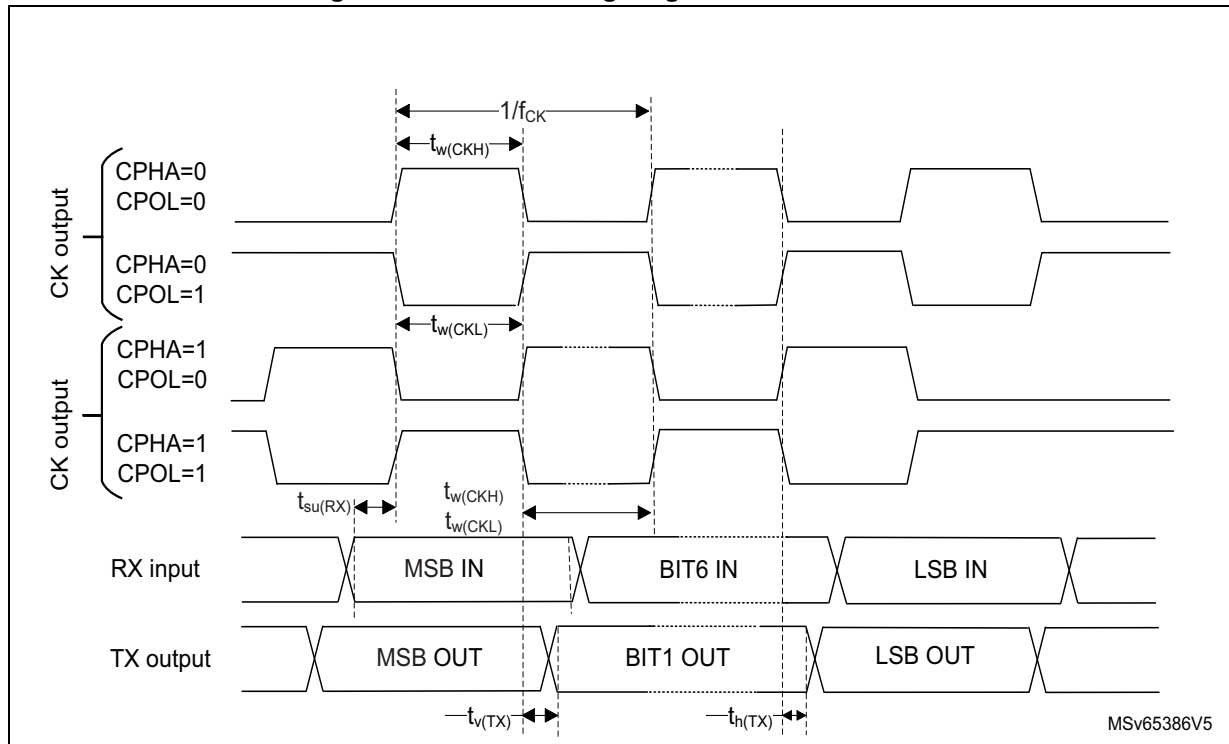
Figure 81. USART timing diagram in master mode
