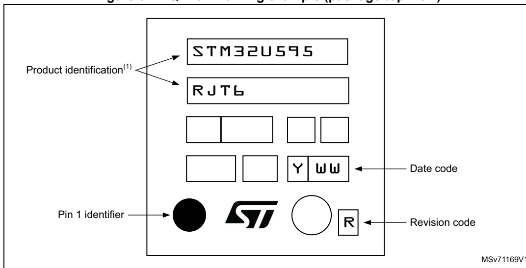
Figure 92. LQFP64 marking example (package top view)
