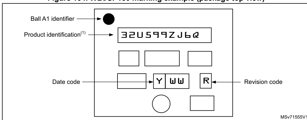
Figure 104. WLCSP150 marking example (package top view)
