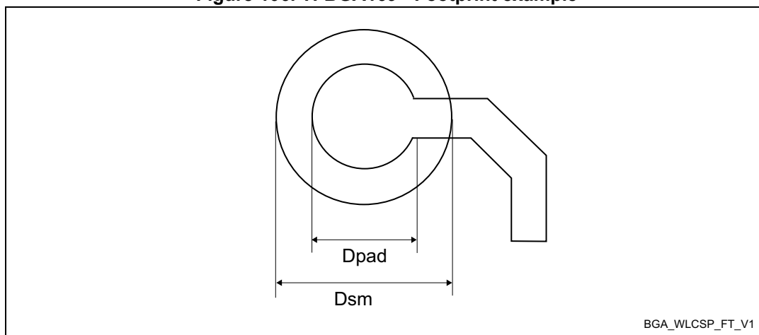
Figure 106. TFBGA169 - Footprint example
