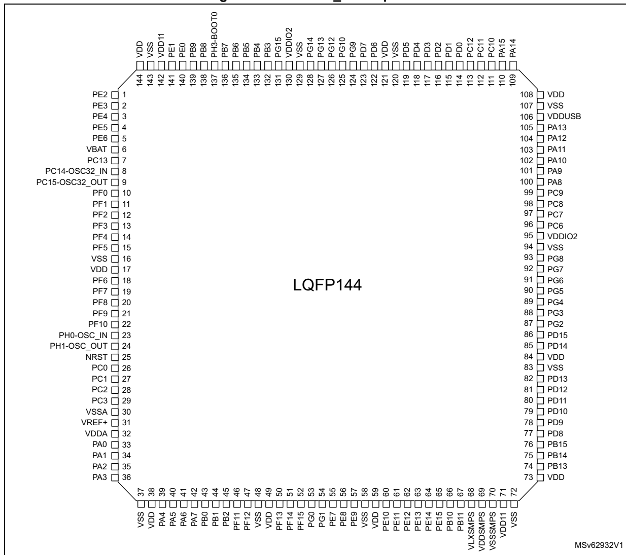
Figure 13. LQFP144_SMPS pinout
