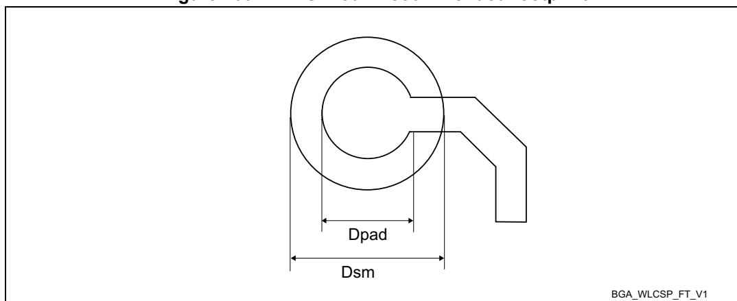
Figure 103. WLCSP150 - Recommended footprint
