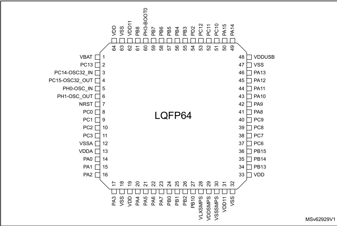
Figure 11. LQFP64_SMPS pinout
