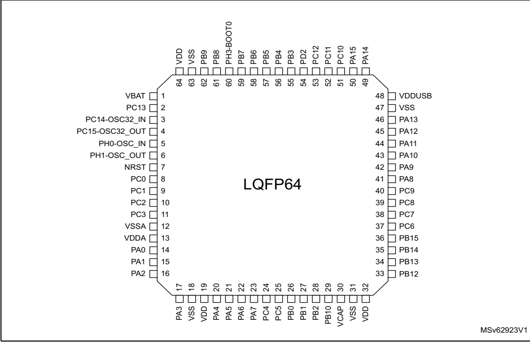
Figure 12. LQFP64 pinout
