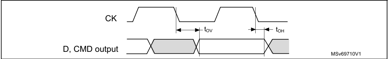
Figure 59. SD default mode
