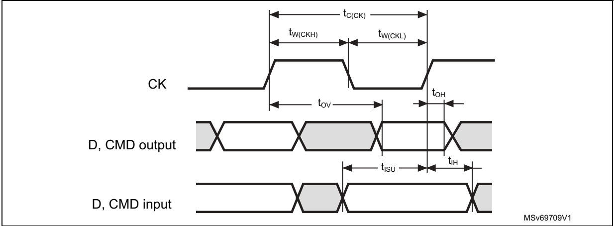
Figure 58. SD high-speed mode
