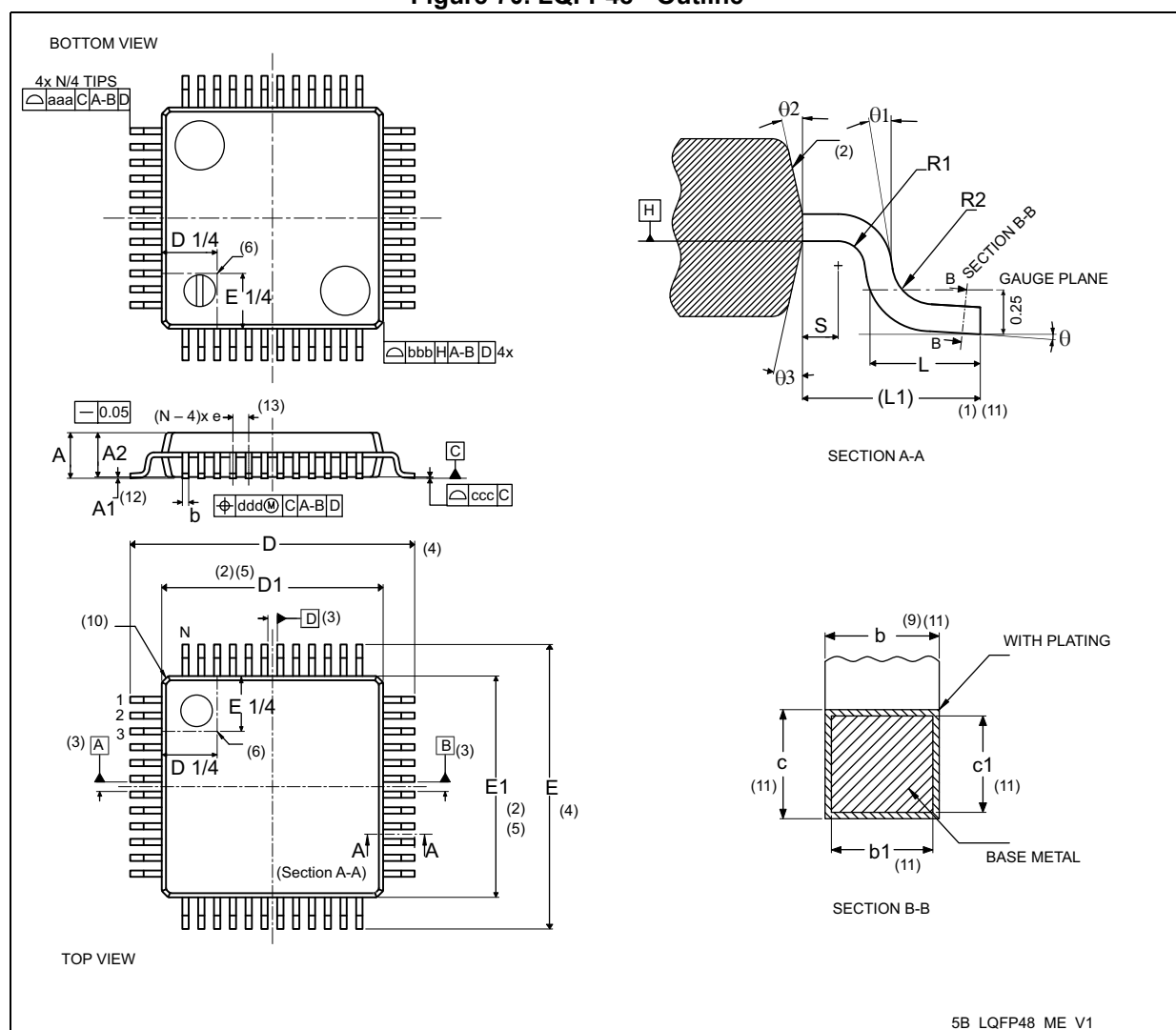
Figure 70. LQFP48 - Outline (15)
