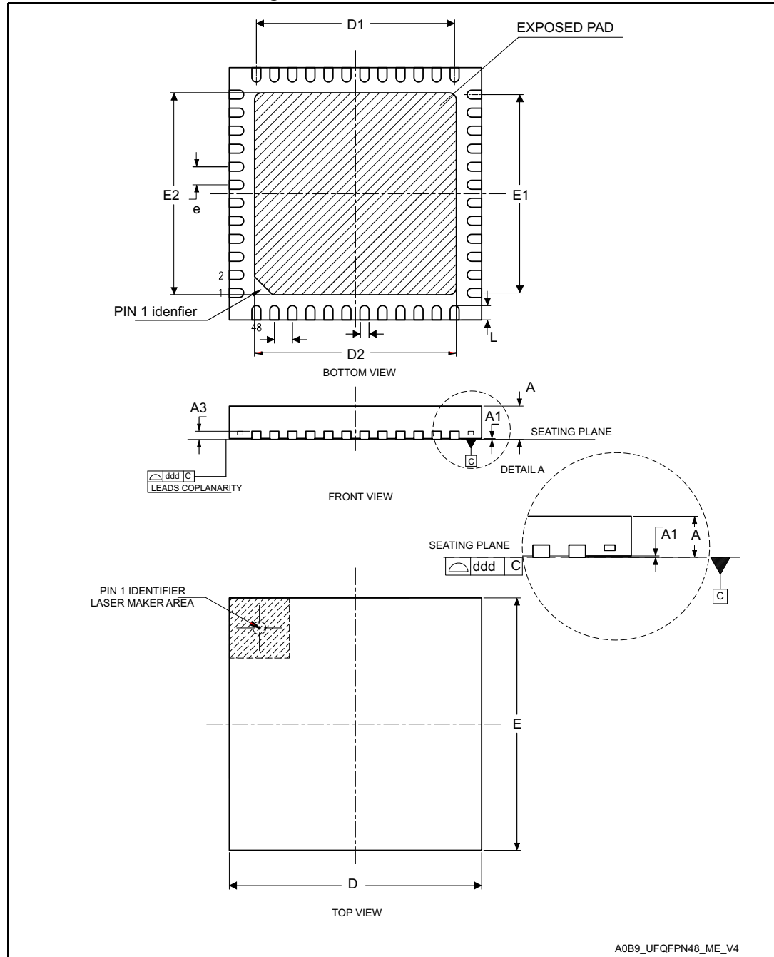
Figure 73. UFQFPN48 – Outline
