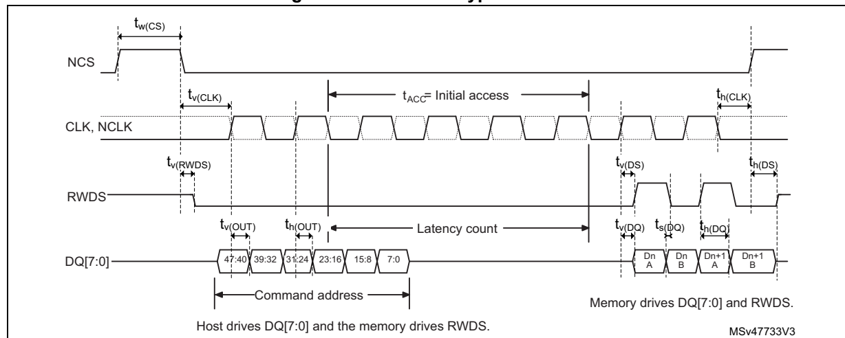
Figure 55. OCTOSPI HyperBus read
