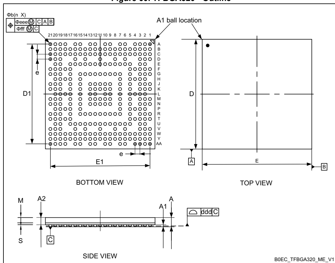
Figure 60. TFBGA320 - Outline
