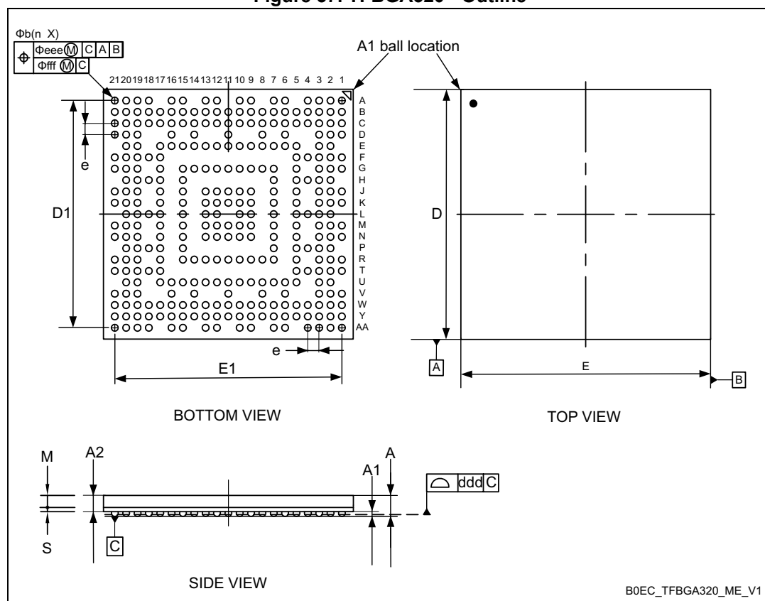
Figure 57. TFBGA320 - Outline
