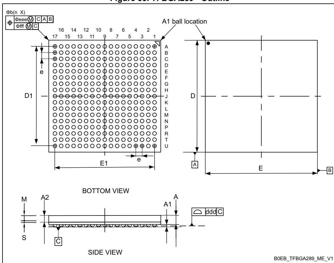
Figure 55. TFBGA289 - Outline
