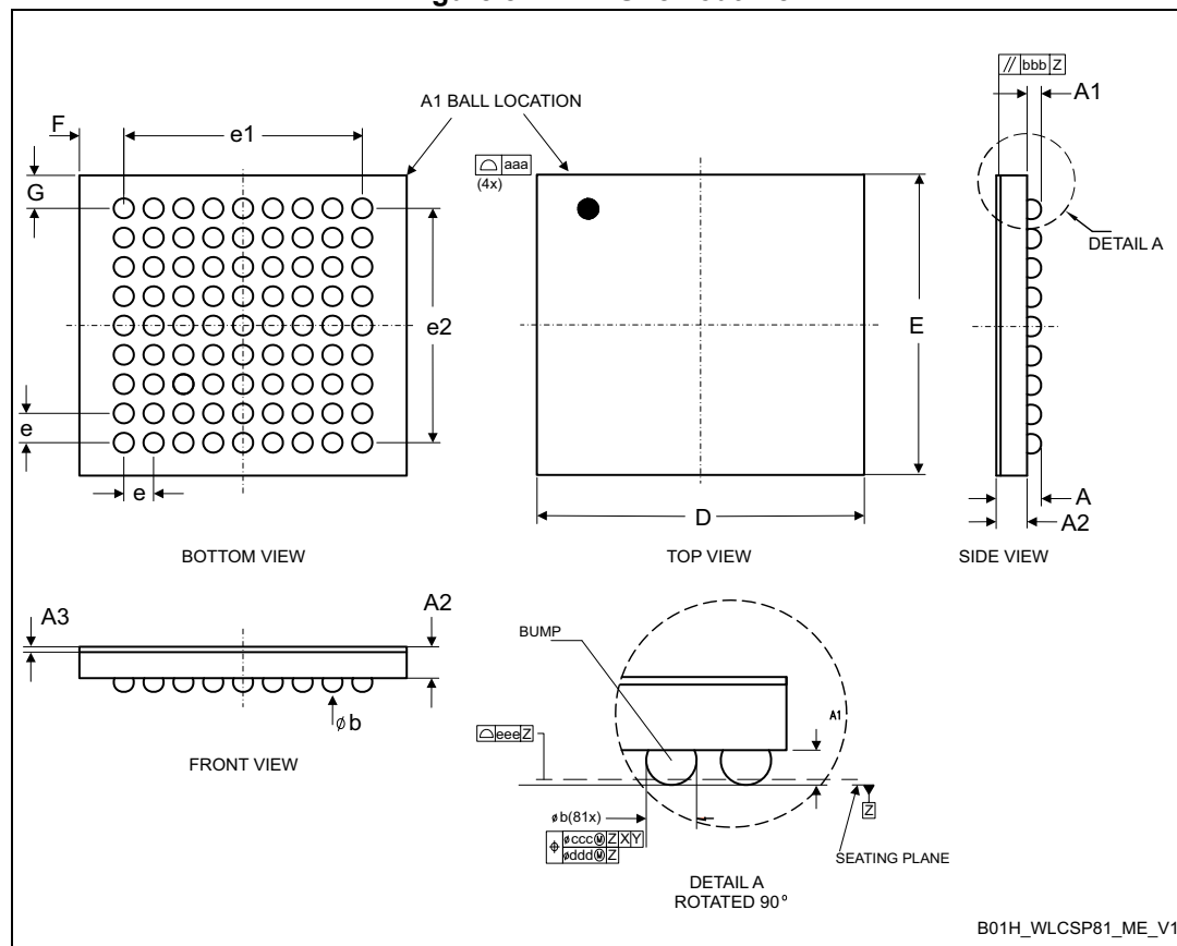
Figure 82. WLCSP81 outline
