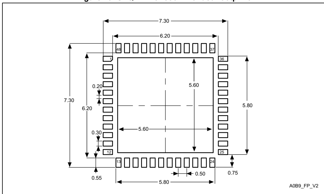
Figure 79. UFQFPN48 recommended footprint
