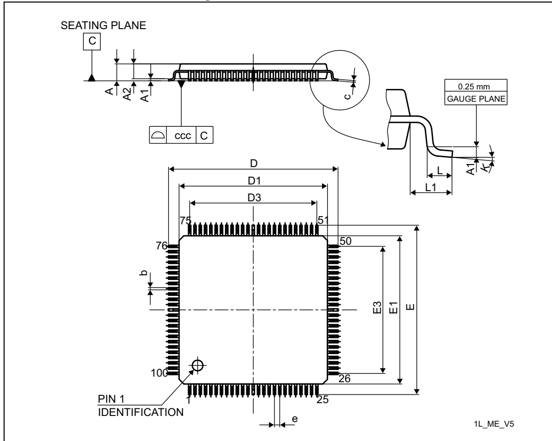
Figure 85. LQFP100 outline
