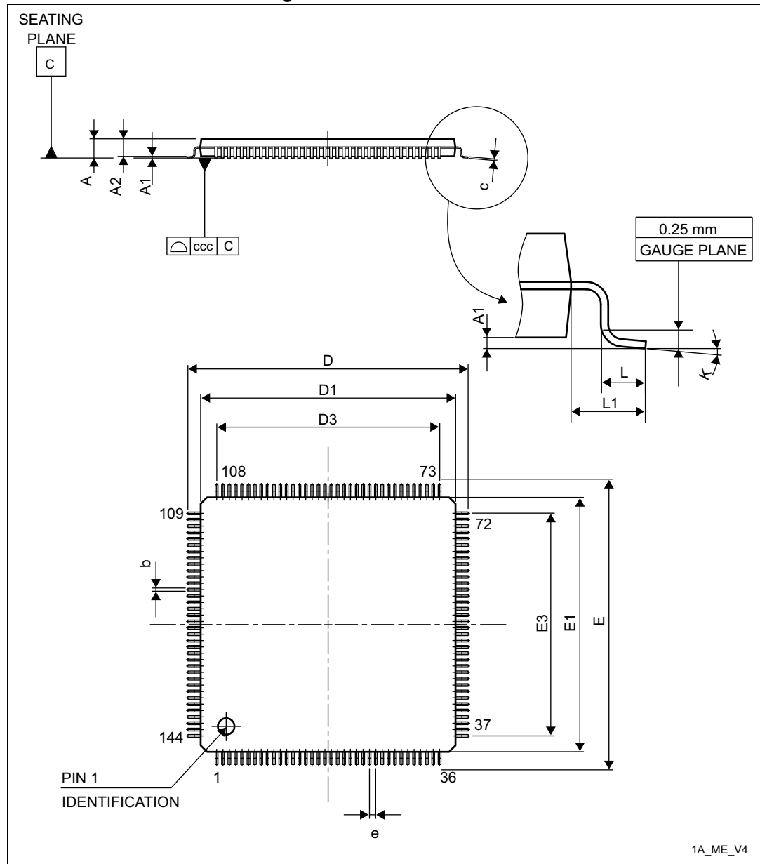
Figure 89. LQFP144 outline
