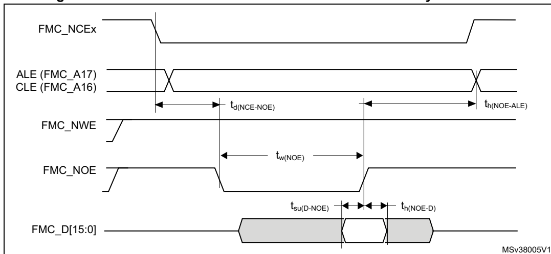
Figure 65. NAND controller waveforms for common memory read access
