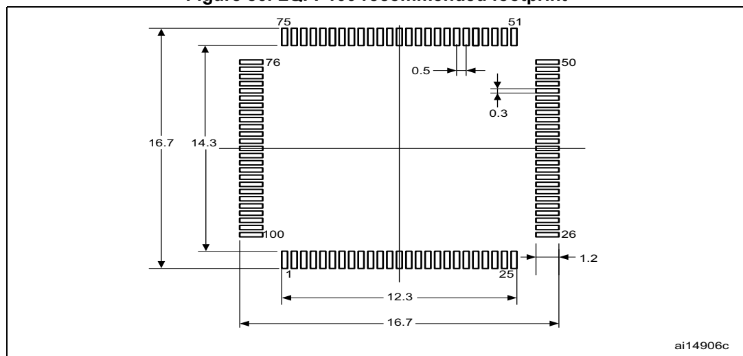
Figure 86. LQFP100 recommended footprint
