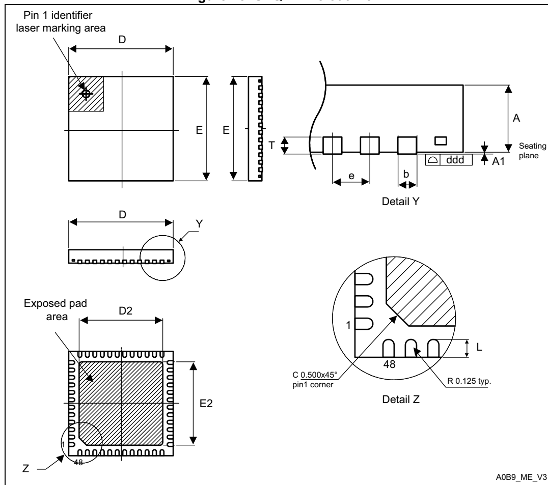
Figure 78. UFQFPN48 outline
