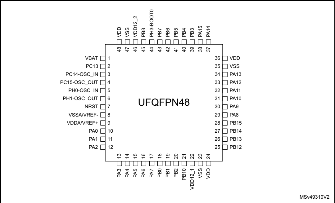
Figure 13. STM32L562xxxxP UFQFPN48 external SMPS pinout
