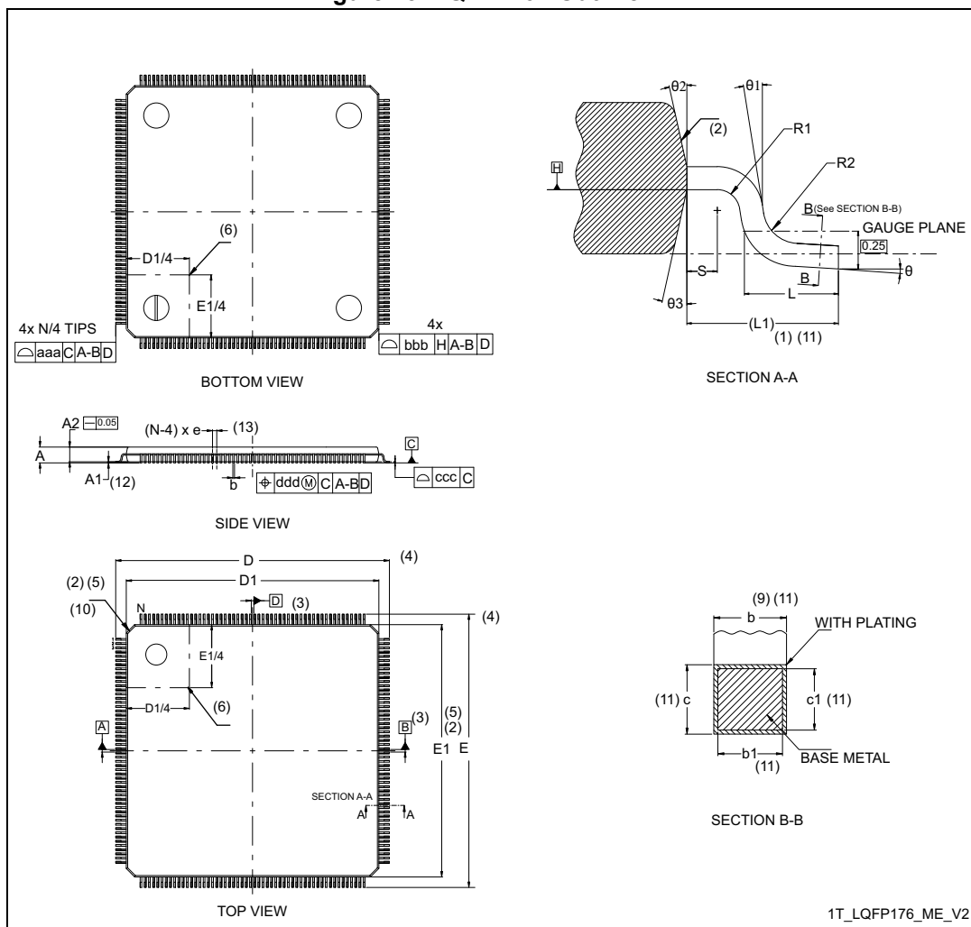
Figure 75. LQFP176 - Outline (15)
