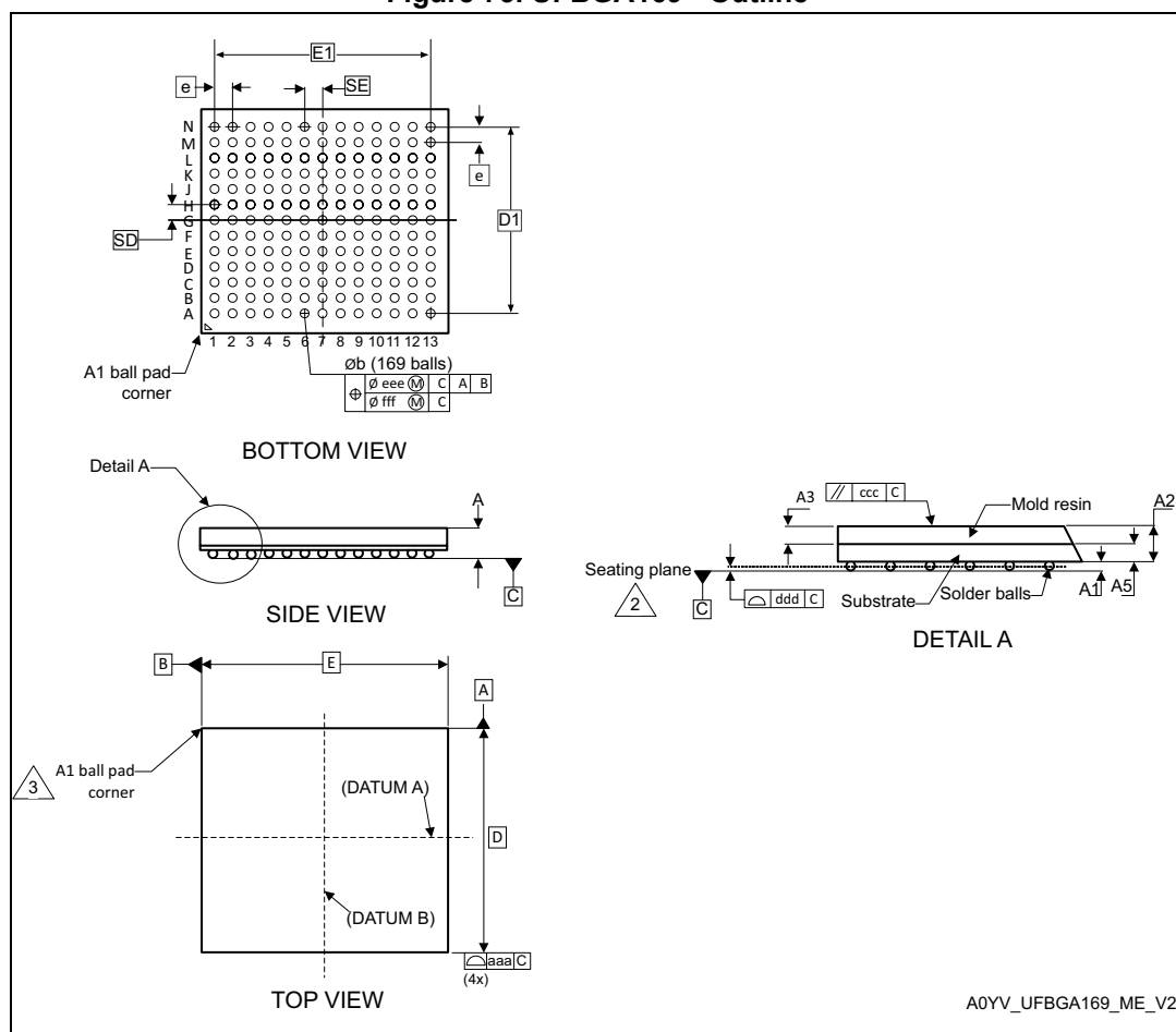
Figure 73. UFBGA169 - Outline
