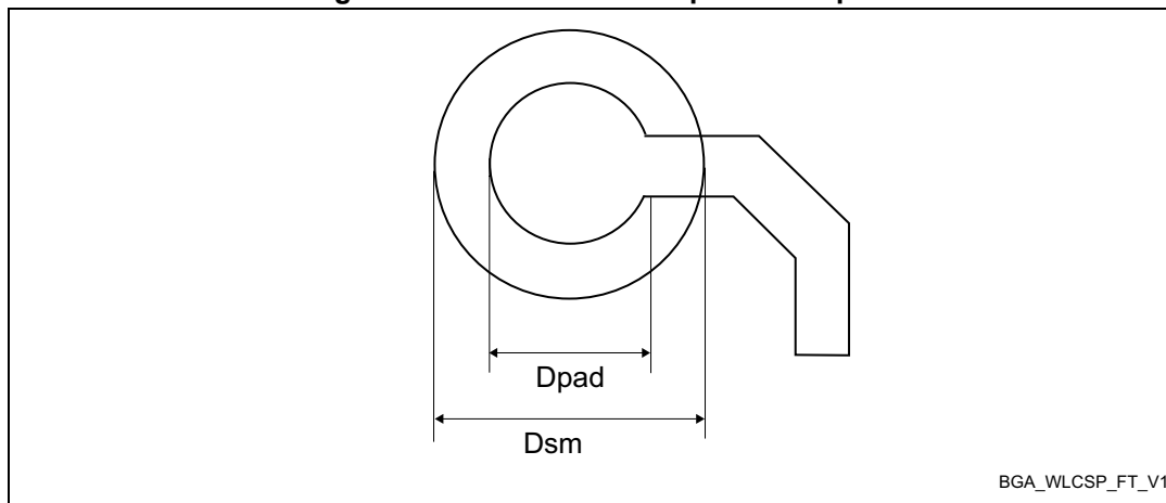
Figure 67. TFBGA100 - Footprint example
