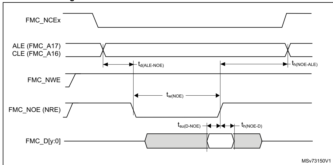
Figure 27. NAND controller waveforms for read access
