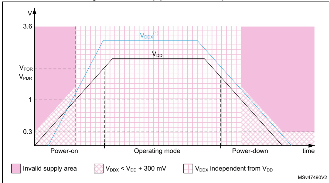
Figure 2. Power-up/power-down sequence
