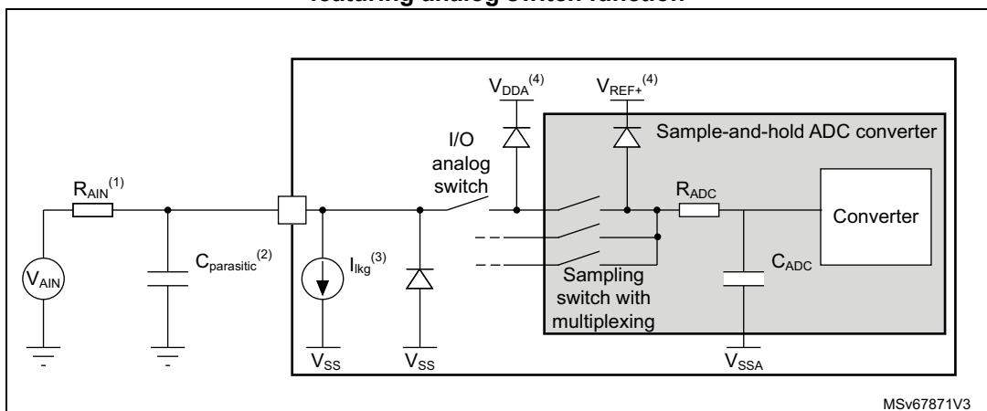
Figure 37. Typical connection diagram when using the ADC with FT/TT pins featuring analog switch function
