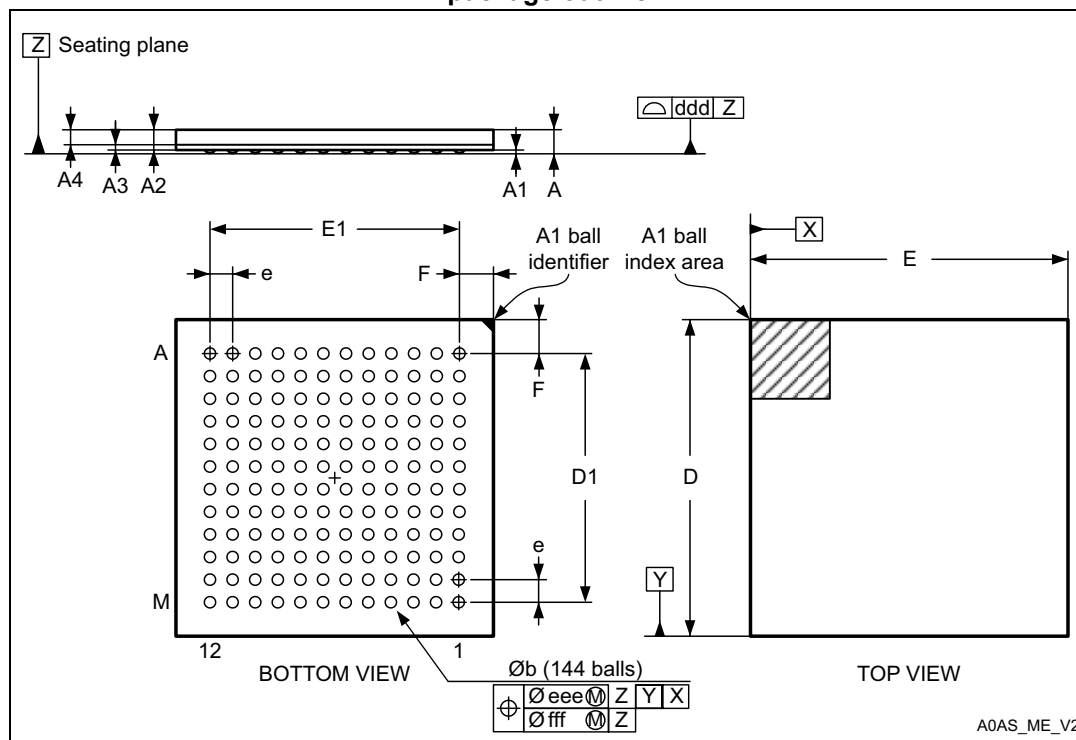
Figure 70. UFBGA - 144 balls, 7 x 7 mm, 0.50 mm pitch, ultra fine pitch ball grid array package outline
