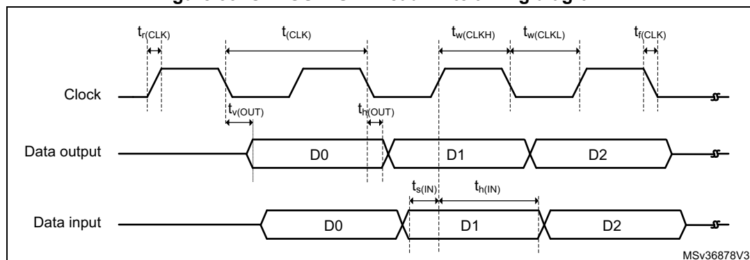
Figure 33. OCTOSPI SDR read/write timing diagram
