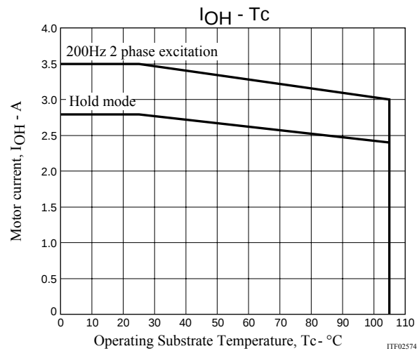
Derating Curve of Motor Current, I_{OH} , vs. STK672-440B-E Operating Substrate Temperature, T_c
