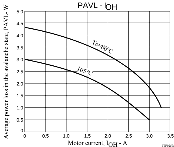
Figure 3 Allowable Loss Range, PAVL-I_{OH} During STK672-440B-E Avalanche Operations
