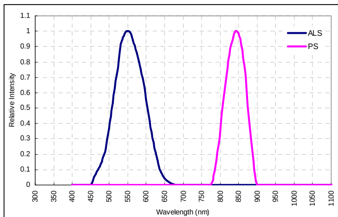
Spectral Response
