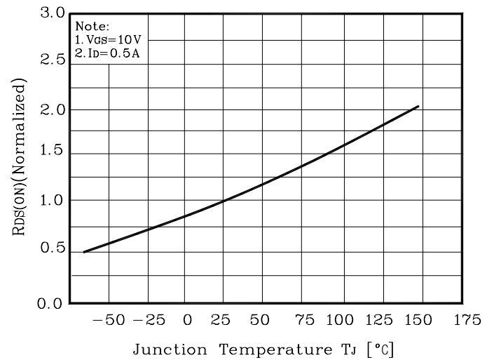
Fig. 8 R_{DS(on)} - T_J
