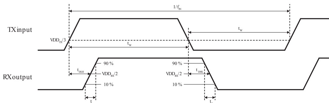
Figure 5. Timing diagram
