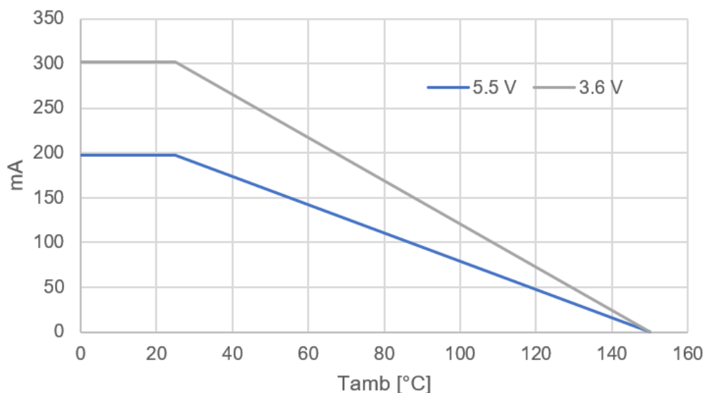
Figure 2. Thermal derating curve for current safety limiting
