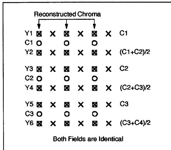
Figure 46 : Derivation of Chrominance in Mode 4
