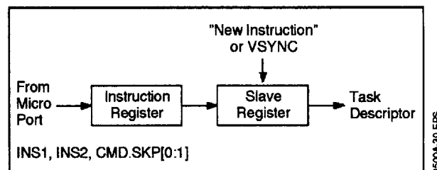
Figure 28 : Instruction Buffering
