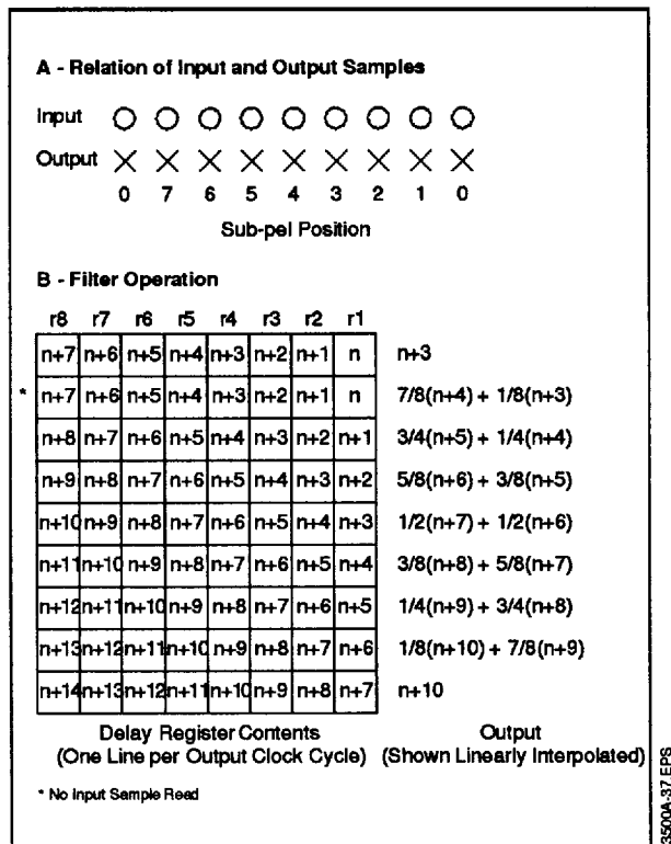
Figure 35 : SRC Example for 8:7 Upsampling
