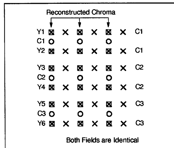
Figure 47 : Derivation of Chrominance in Mode 5
