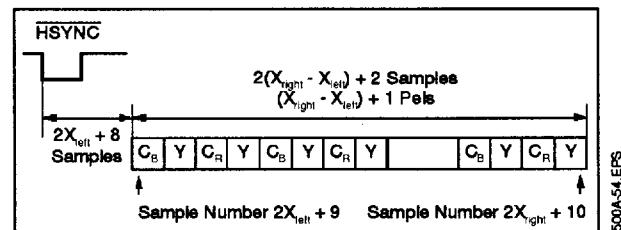
Figure 52 : OSD Region Horizontal Positioning
