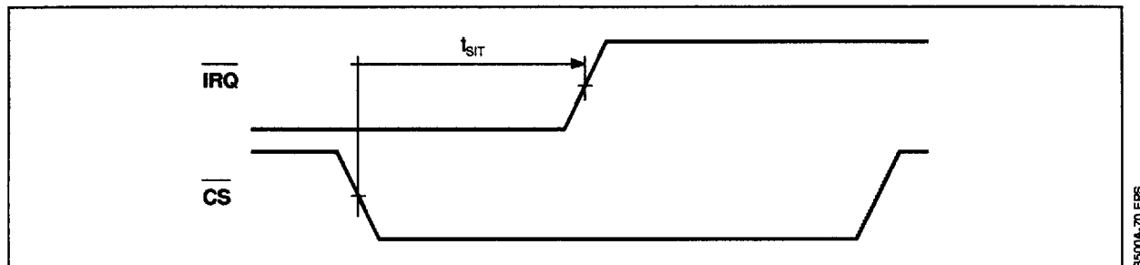
Figure 68 : Interrupt Acknowledge
