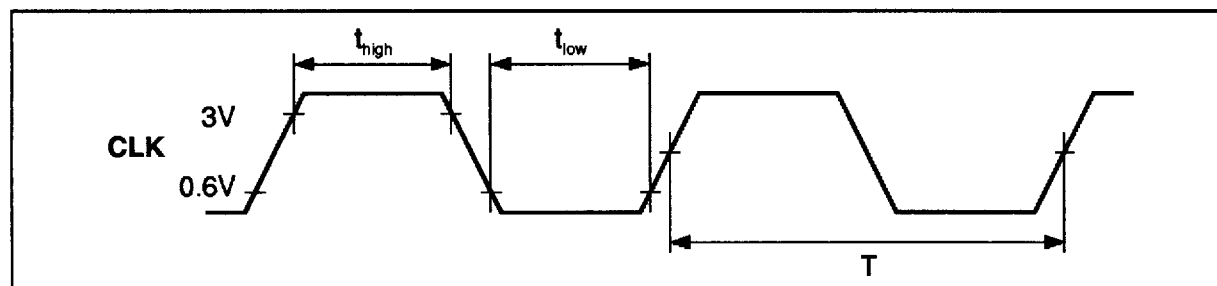
Figure 64 : Primary Clock
