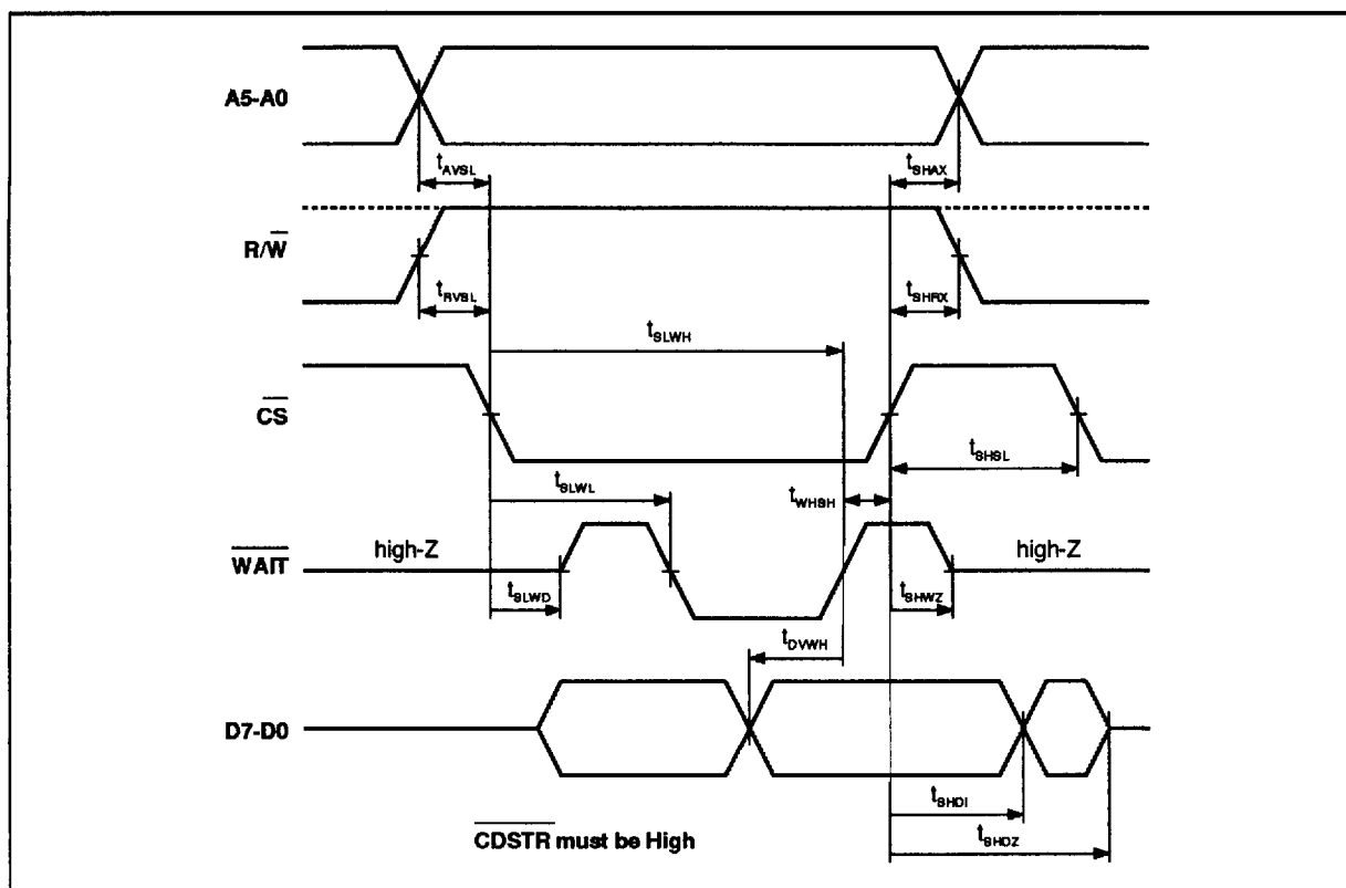
Figure 66 : Two-Byte Register Read Cycle
