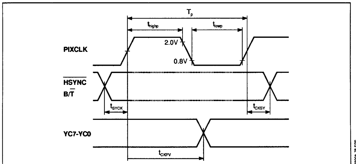
Figure 73 : Video Interface
