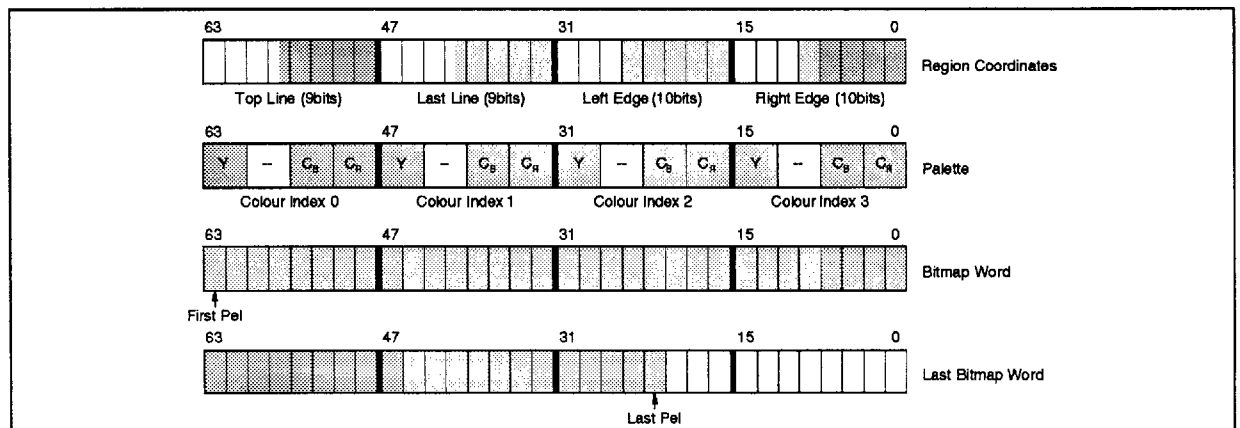
Figure 51 : OSD Region Specification Word Formats
