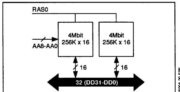
Figure 18 : 8Mbit Memory Configuration
