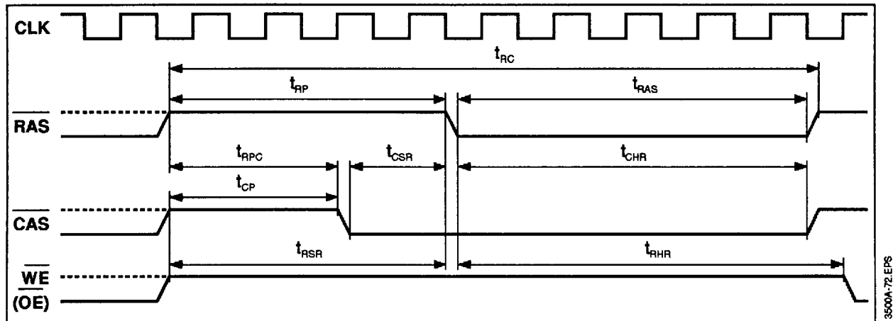
Figure 70 : \overline{\text{CAS}} Before \overline{\text{RAS}} Refresh Cycle
