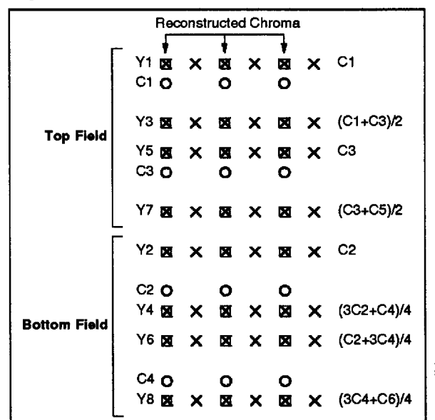
Figure 42 : Derivation of Chrominance in Mode 0
