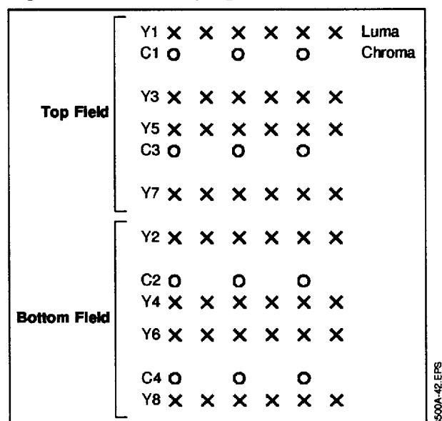
Figure 40 : Field Sampling Patterns
