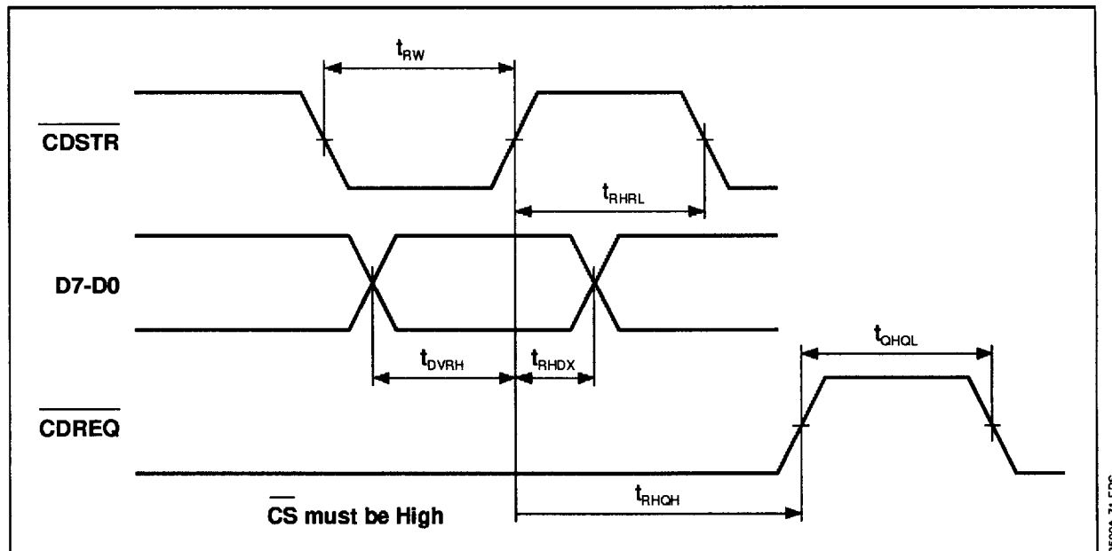
Figure 69 : Compressed Data Write
