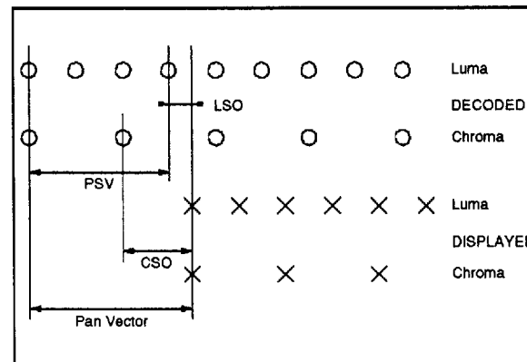
Figure 39 : Components of the Pan Vector
