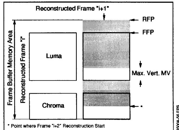
Figure 54 : Memory Reuse in 8-Mbit mode
