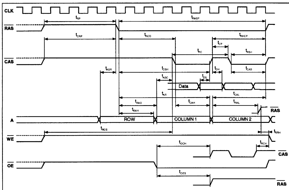
Figure 71 : Page Mode Read Cycle
