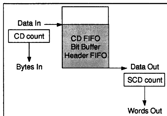
Figure 27 : Bit Buffer Read and Write Counters
