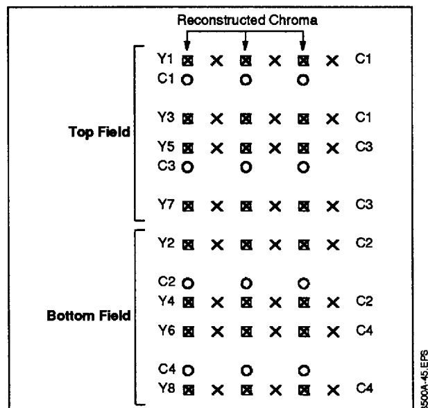
Figure 43 : Derivation of Chrominance in Mode 1
