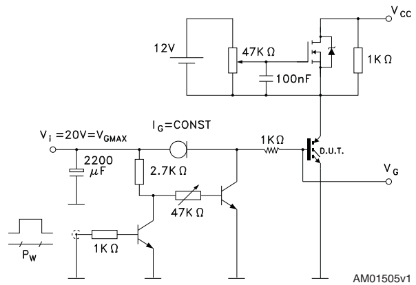
Figure 30. Gate charge test circuit
