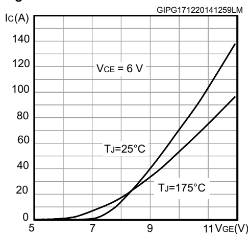
Figure 10. Transfer characteristics
