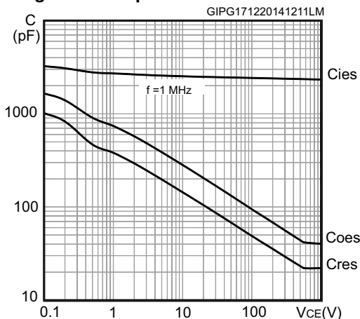
Figure 14. Capacitance variations
