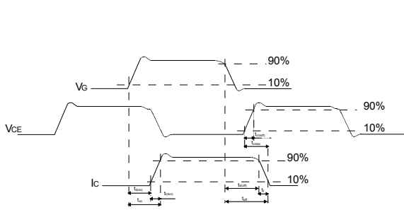
Figure 19. Switching waveform
