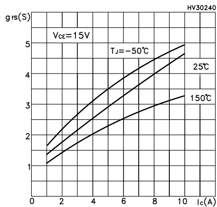
Figure 3. Transconductance
