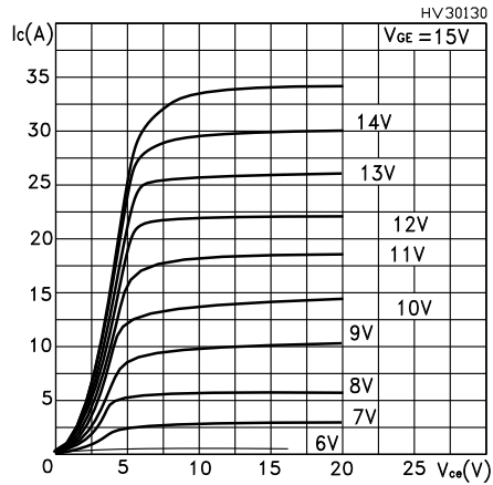
Figure 1. Output characteristics
