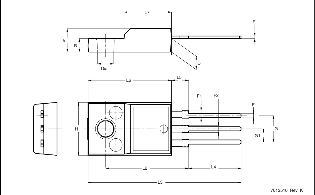
Figure 22. TO-220FP drawing
