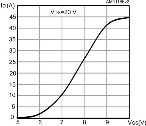
Figure 9: Transfer characteristics
