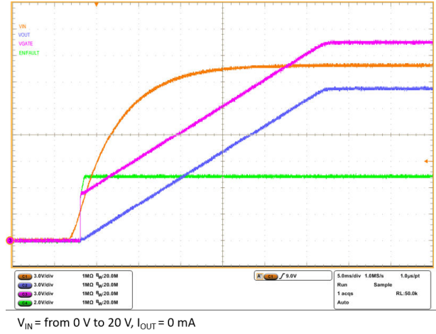
Figure 27. Startup into voltage clamp
