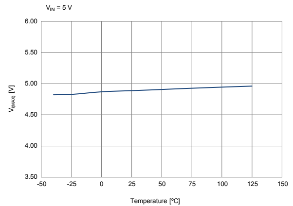
Figure 21. EN/Fault pull-up voltage vs. temperature
