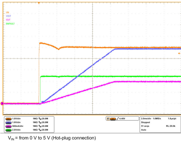
Figure 26. Startup with R_{LOAD} = 5\ \Omega
