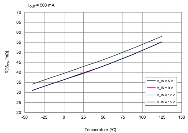
Figure 15. R_{DS\_ON} vs. temperature
