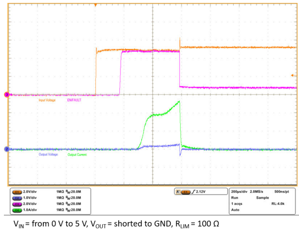
Figure 29. Start-up into output short-circuit
