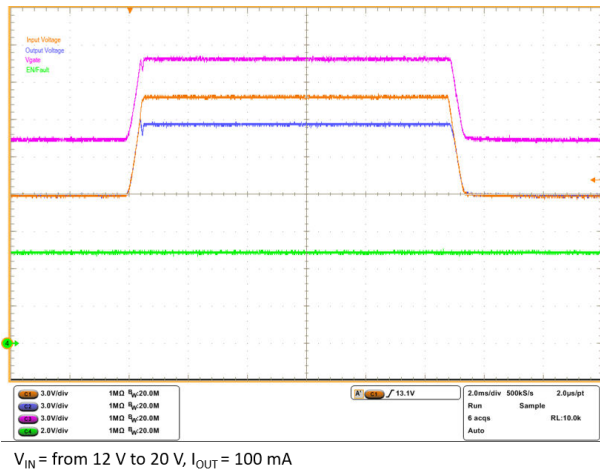
Figure 28. Voltage clamp during operation
