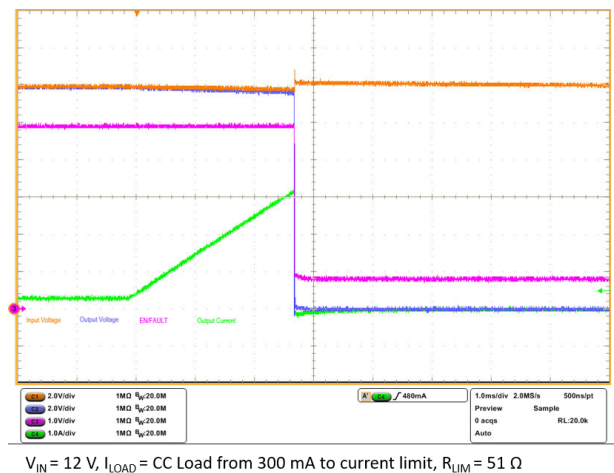
Figure 31. Overcurrent protection during operation (latched version)
