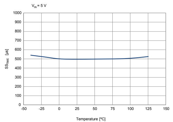
Figure 23. Soft-start time vs. temperature (no Cdv/dt)
