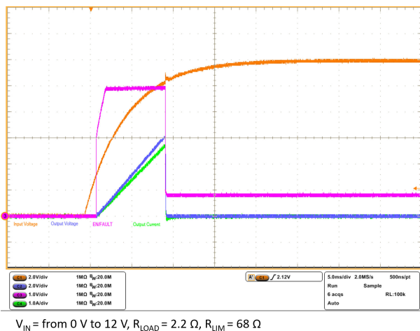
Figure 30. Start-up into overload
