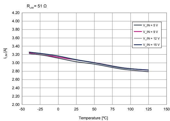
Figure 16. I_{LIM} vs. temperature
