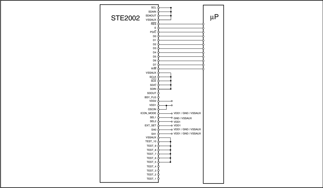
Figure 37. Host processor interconnection with parallel interface
