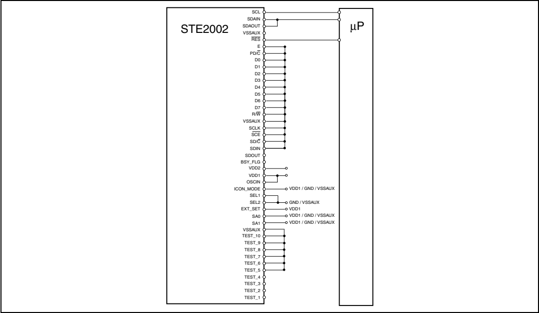
Figure 35. Host processor interconnection with I2C interface
