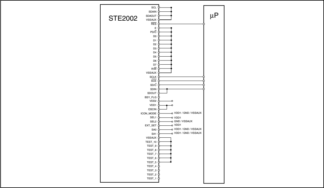
Figure 36. Host processor interconnection with serial interface
