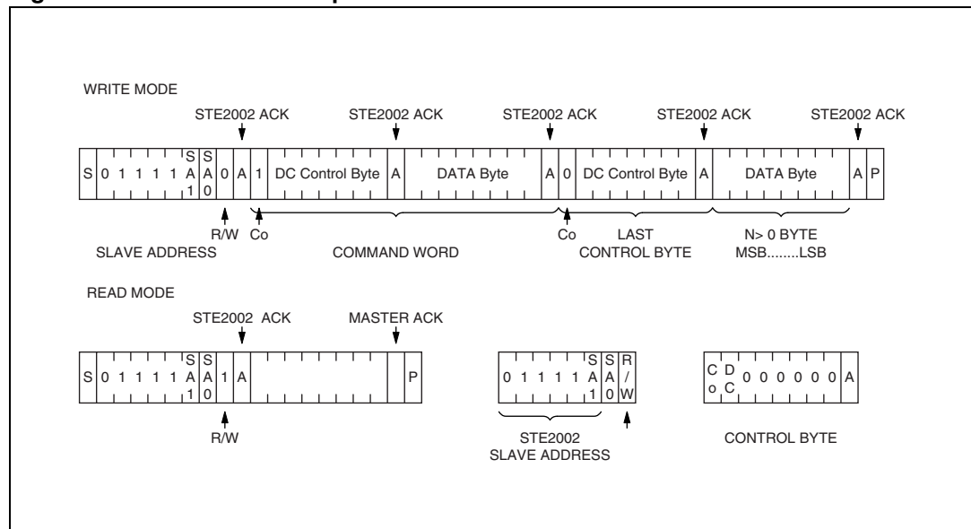
Figure 30. Communication protocol
