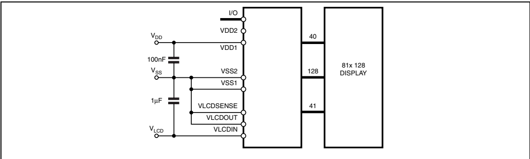
Figure 38. application schematic using an external lcd Voltage Generator
