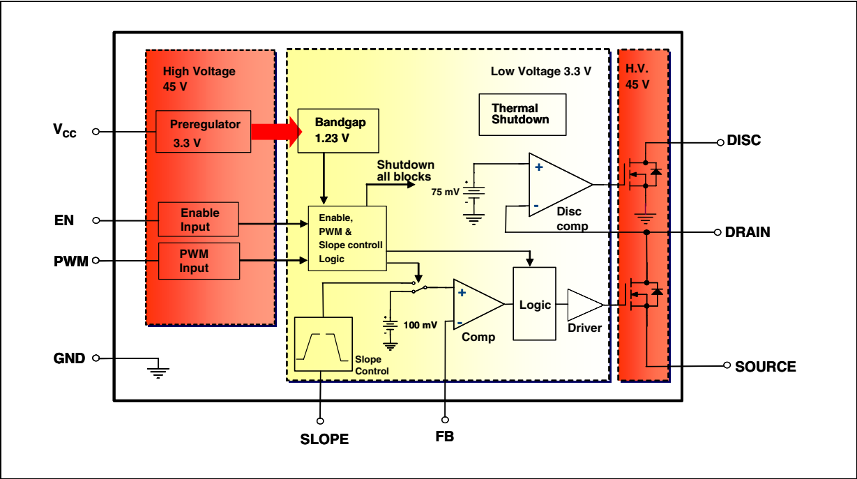
Figure 4. Block diagram
