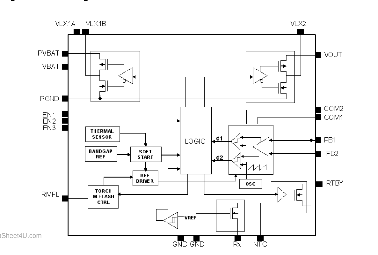
Figure 3. Block diagram
