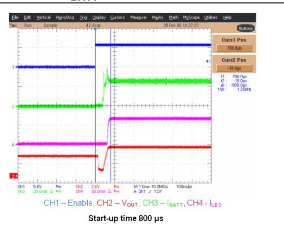
Figure 9. Start-up to torch mode 25 mA at V_{BATT} = 3.6V
