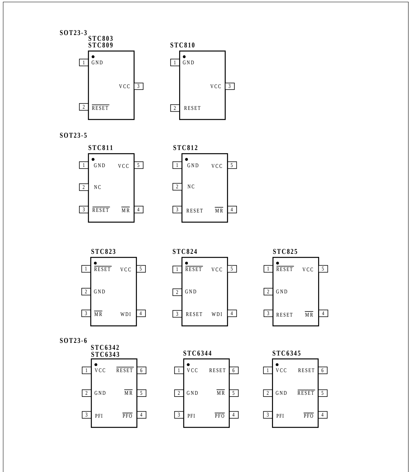
Figure 2. Pin Configuration
