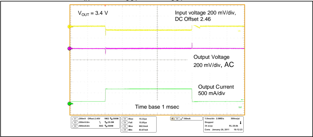
Figure 15. V_{IN} = 4.2 V , V_{OUT} = 3.4 V , I_{OUT} = from 80 mA to 1100 mA
