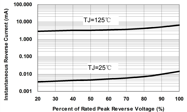
Fig.2-Typical Reverse Characteristics
