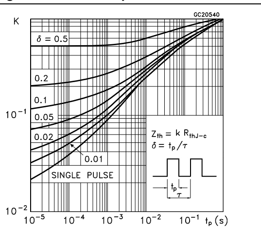
Figure 3. Thermal impedance for D 2 PAK
