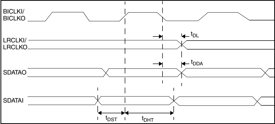
Figure 7. Master mode
