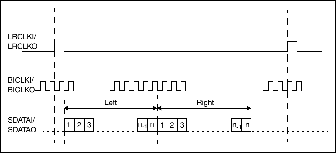
Figure 11. DSP
