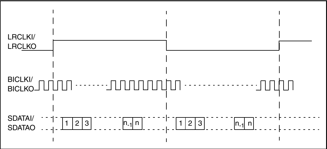
Figure 12. I 2 S
