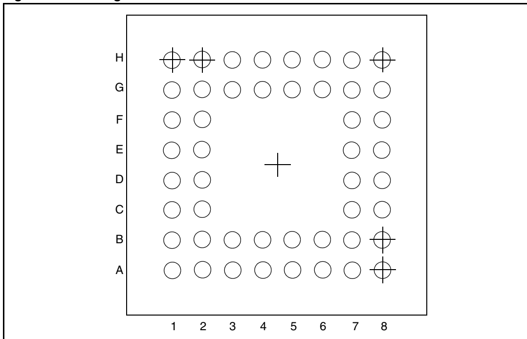
Figure 2. Package: TFBGA48
