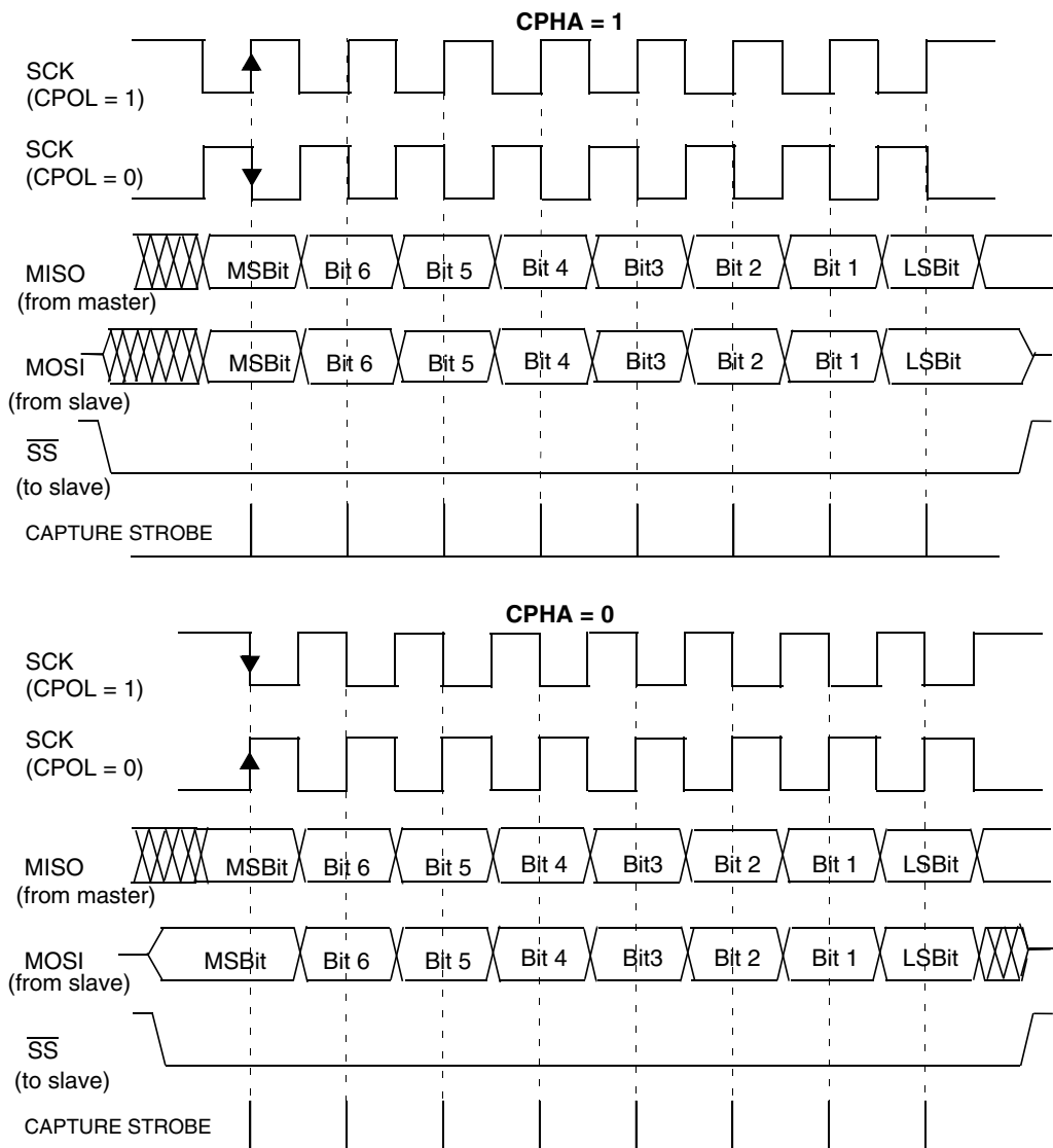
Figure 54. Data Clock Timing Diagram
