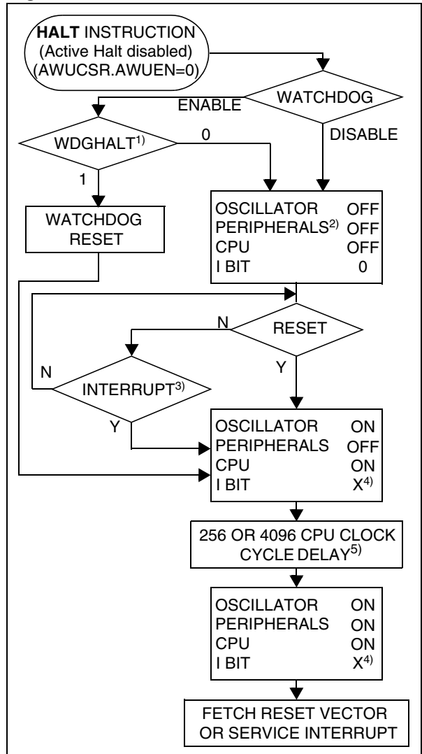
Figure 23. HALT Mode Flowchart
