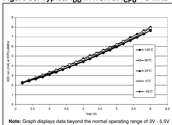
Figure 68. Typical I_{DD} in RUN at f_{CPU} = 8\text{ MHz}
